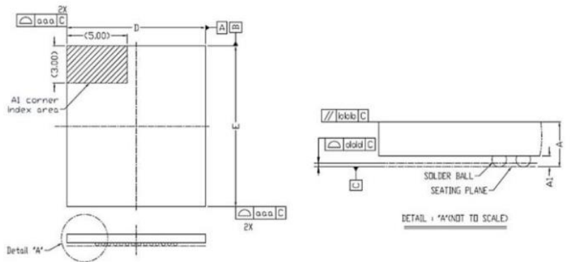
Package Outline Drawing - Top and Side View
