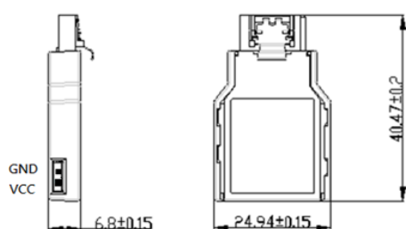
Vertical (without housing)
